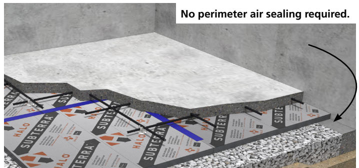
Subterra or Subterra Plus installed as a vapor barrier.
