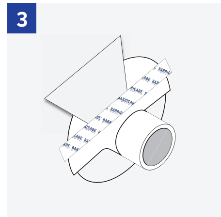
3 Replace building wrap flap over the flashing and tape across using Barricade Seam Tape.
