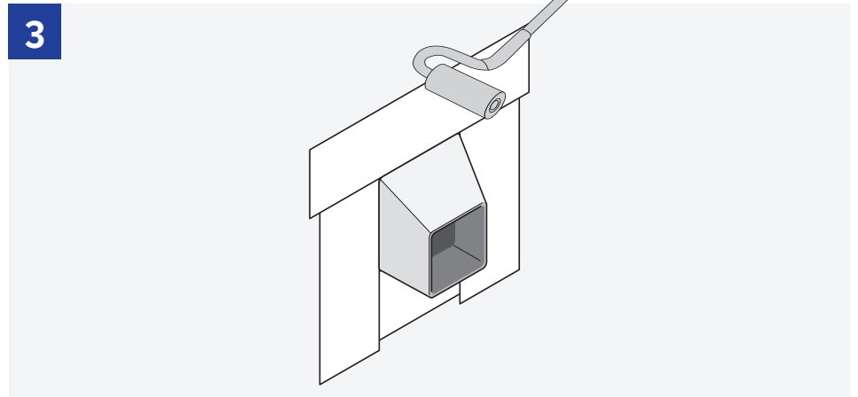
3 Use a roller to apply even pressure along the flashing, being sure to push out any air pockets that may have appeared. Barricade suggests finishing with Barricade Construction Sealant to ensure a tight seal around the edges of the penetration.
