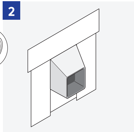
2 Apply Barricade Window flashing along the sides and then the top, shingling each layer.
