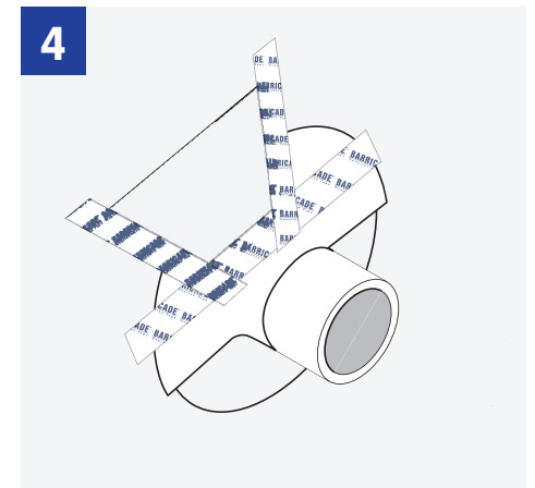
4 Tape over the 45° cuts using Barricade Seam Tape.
