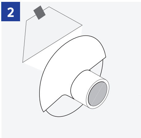
2 Apply Barricade Flash Conform to the underside of penetration, shingling the above side after. Use a roller to apply even pressure along the flashing.
