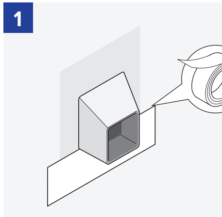
1 Apply Barricade Window flashing to the bottom of the penetration.
